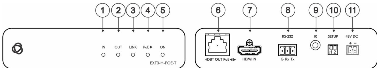
Figure 1: EXT3-H-POE-T Transmitter
