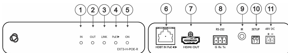
Figure 2: EXT3-H-POE-R Receiver
